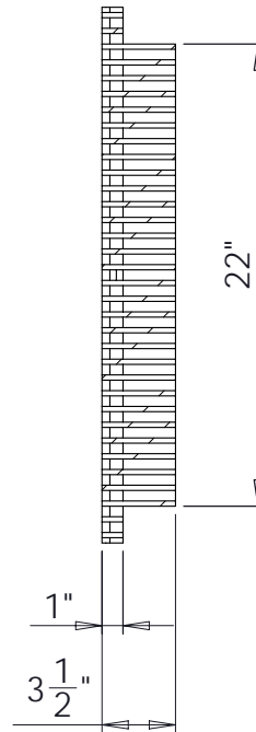
SECTION B-B
